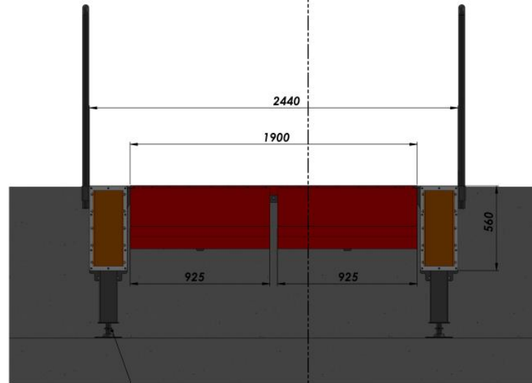
ADJUSTABLE LEG
